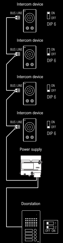
Intercom device
